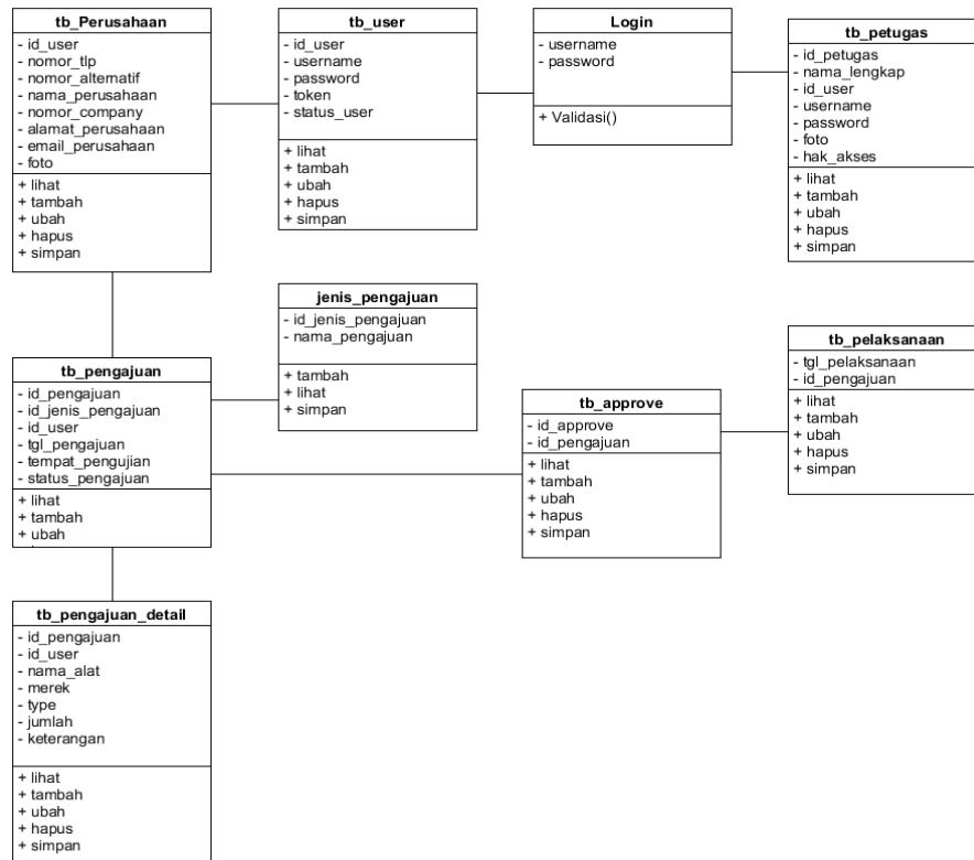
Gambar 5. Relasi Diagram
